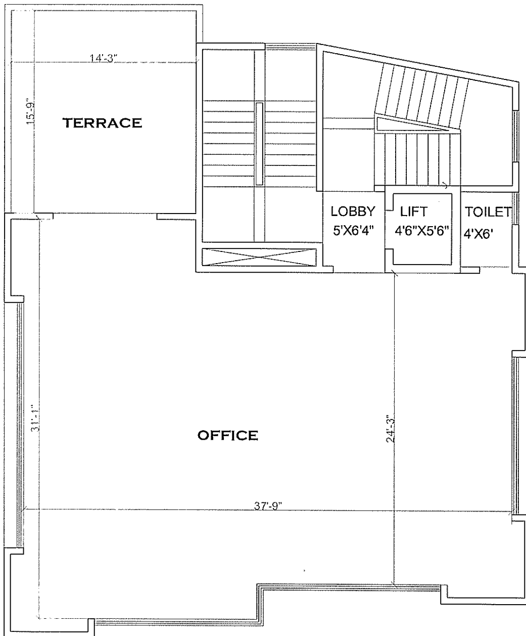
FOURTH FLOOR
