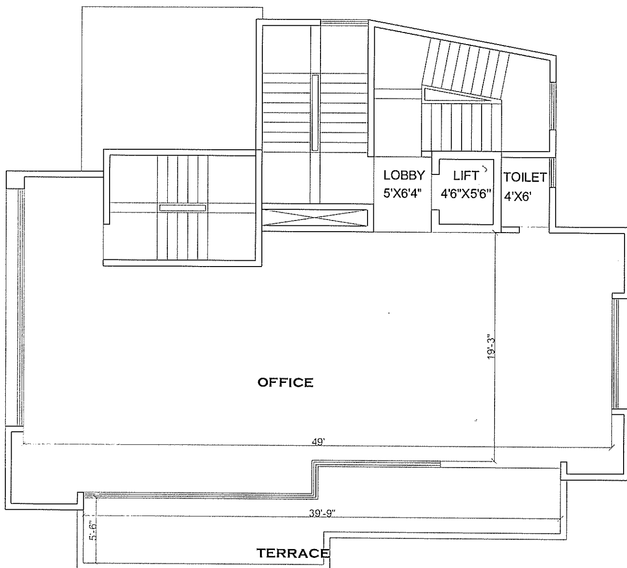
FIFTH FLOOR
