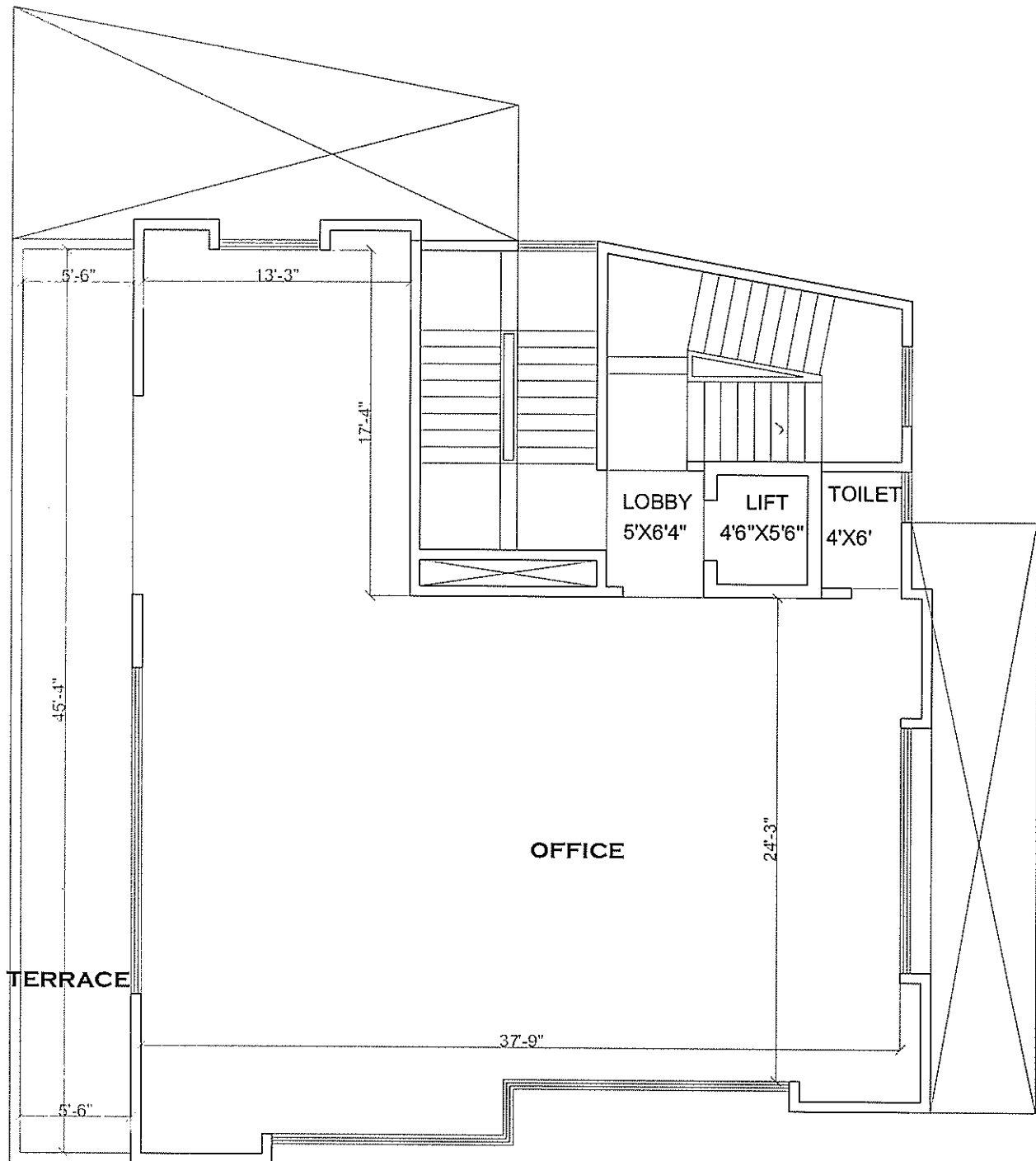
THIRD FLOOR
