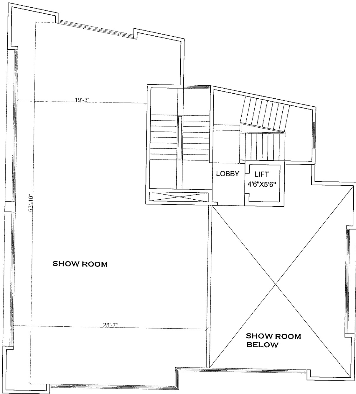
MEZZANINE FLOOR
